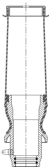
110 01 C Cabin air spring without shock absorber
