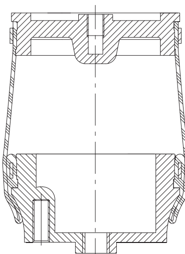
210 06 C Seat air springs
