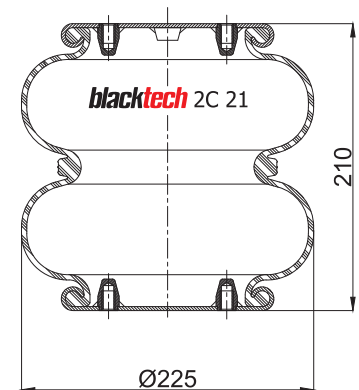
2C 21 - 210 P13 With crimped baead plate or with steel bead ring and the mounting plate
