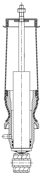
110 01 CA Cabin air spring with shock absorber plates
