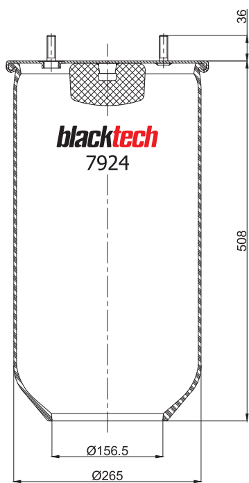
RML 7924 Air spring system without piston
