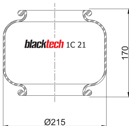
1 C1 21 - 170 S Rubber Bellow Only
